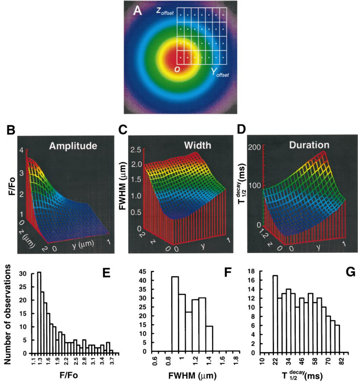
FIGURE 5 Effects of random off-center sampling on experimental parametric measurement of stereotypical \text{Ca}^{2+} sparks. ( A ) Position of scan lines in relation to \text{Ca}^{2+} sparks. Side view of scan lines ( crosses ) running across \text{Ca}^{2+} sparks ( shaded areas ) originated at point O. Direction of linescan is perpendicular to the section plane. A scan line can run right through the spark origin, or more likely, be displaced either laterally ( Y_{\text{offset}} ), or vertically ( Z_{\text{offset}} ), or in both directions. If the scanning line is positioned randomly with respect to the origin of the \text{Ca}^{2+} spark and the spark is spherically symmetric, we expect the distribution of linescan locations to be uniformly distributed across the section plane. ( B–D ) Surface plots of spark amplitude ( B ), width at peak F/F_0 ( C ) and half-decay time, T_{1/2}^{\text{decay}} ( D ) as a function of scan line position ( y, z ). ( E–G ) Histogram distributions of spark parameters after random sampling. As shown in panel A , the scan line was placed at regular, discrete locations, with Y_{\text{offset}} and Z_{\text{offset}} varying from 0–1 \mu\text{m} and 0–2 \mu\text{m} at increments of 0.05 \mu\text{m} and 0.1 \mu\text{m} , respectively. A spark was calculated at each location and the statistics shown are for sparks after thresholding at F/F_0 = 1.25 . Plots are for F/F_0 ( E ), FWHM ( F ), and T_{1/2}^{\text{decay}} ( G ).
