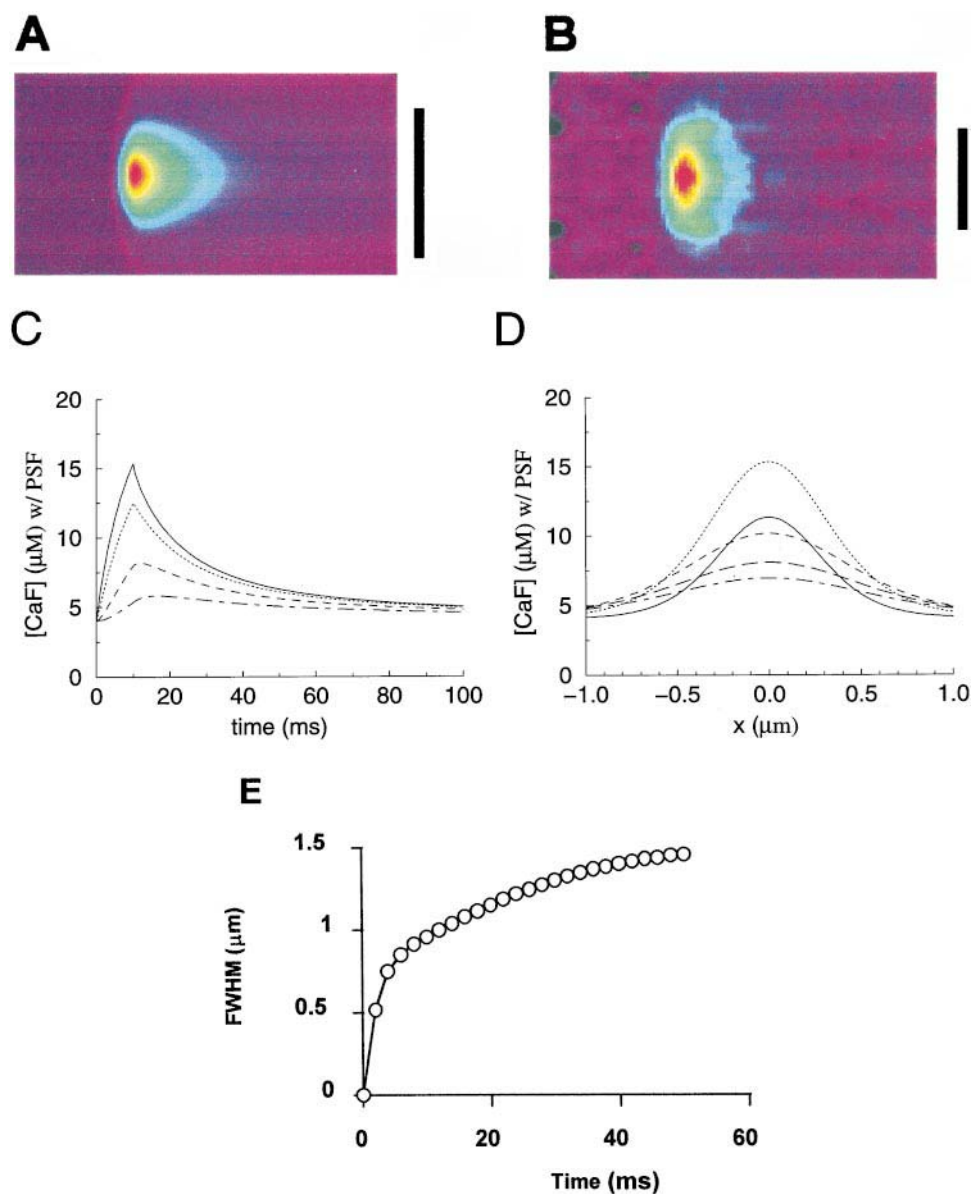
FIGURE 1 Properties of model \text{Ca}^{2+} spark. ( A ) Simulated and ( B ) experimental linescan image of \text{Ca}^{2+} sparks. To produce the image in panel B , 12 sparks from rat ventricular myocytes are aligned and averaged twice by adding their original images and their spatially reversed images. Scale bars: 2 \mu\text{m} . Time: 200 ms from left to right. ( C ) Simulated confocal spot recording of time courses of the model \text{Ca}^{2+} spark at different degrees of offset. From top to bottom, Y_{\text{offset}} = 0.0, 0.25, 0.5, \text{ and } 0.75 \mu\text{m} ; Z_{\text{offset}} is zero. ( D ) Fluorescence ( [\text{CaF}] ) profiles at five different times after the beginning of an in-focus ( Y_{\text{offset}} = Z_{\text{offset}} = 0.0 \mu\text{m} ) \text{Ca}^{2+} release event which occurs at t = 0 . In ms: t = 5 (solid line), 10 (dotted line), 20 (dashed line), 30 (long-dashed line), and 40 (dot-dashed line). ( E ) Spark breadth (FWHM) as a function of time. For simulations in panels A and E , Y_{\text{offset}} = 0.5 \mu\text{m} and Z_{\text{offset}} = 0 . All other parameters used are listed in Tables 1 and 2. After \text{Ca}^{2+} release terminates ( t > 10 ms), the time course of the square of the FWHM gives an apparent diffusion coefficient for \text{Ca}^{2+} of 31 \mu\text{m}^2/\text{s} (not shown).
